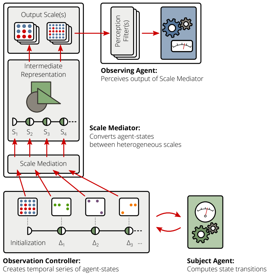
Figure 4.1: Overview of observation components in Thinklab.
