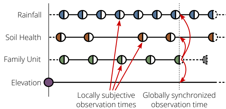
Figure 4.4: Agent observations using globally synchronous, locally subjective time scales
